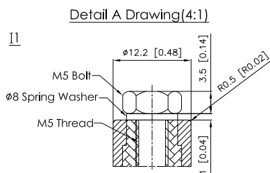
[M5 Bolt & M5 Thread & Spring Washer]
